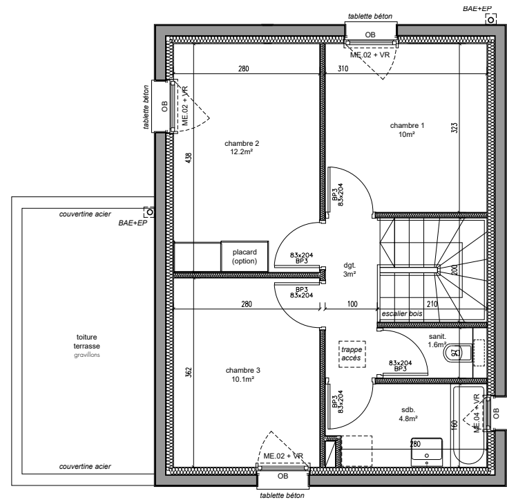
Plan R+1 - 1/100'
