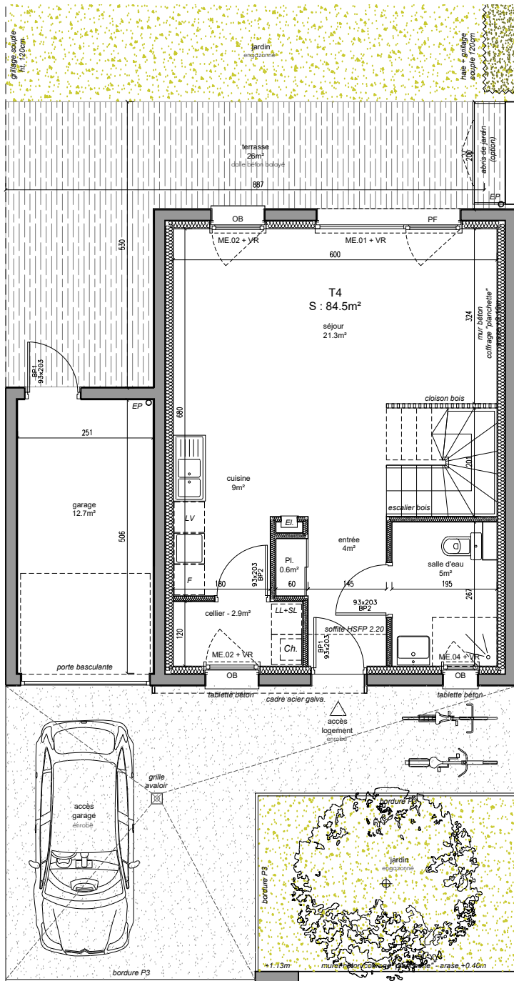
Plan RDC - 1/100'
